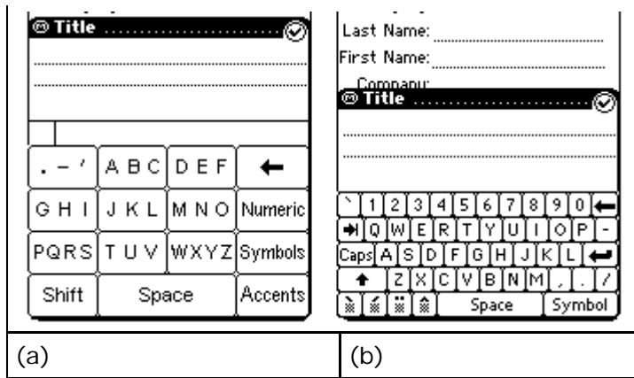
Figure 1. Pictorial representation of the (a) T9 and (b) QWERTY keyboards.
